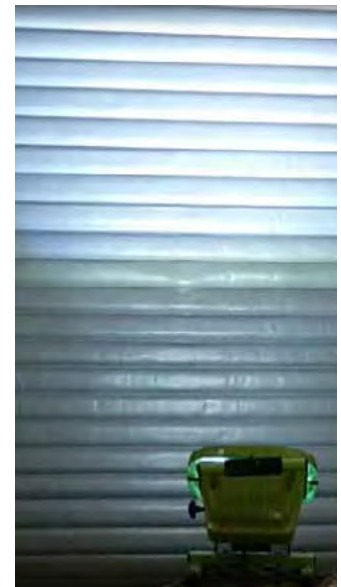
| Fibershield -/60/60 unique barrier provides full insulation equivalent to a fire resistant wall when fully deployed
